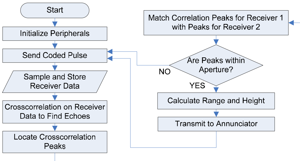
Figure 29: Sensor board program overview flowchart.
